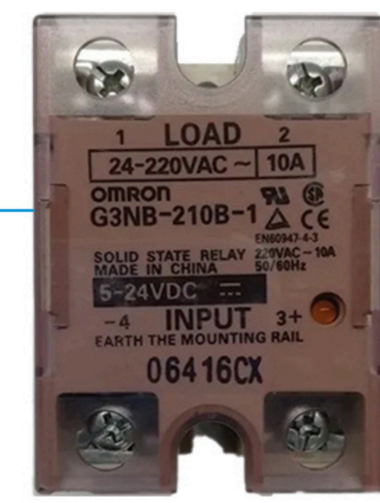
Solid State Relay (SSR)
